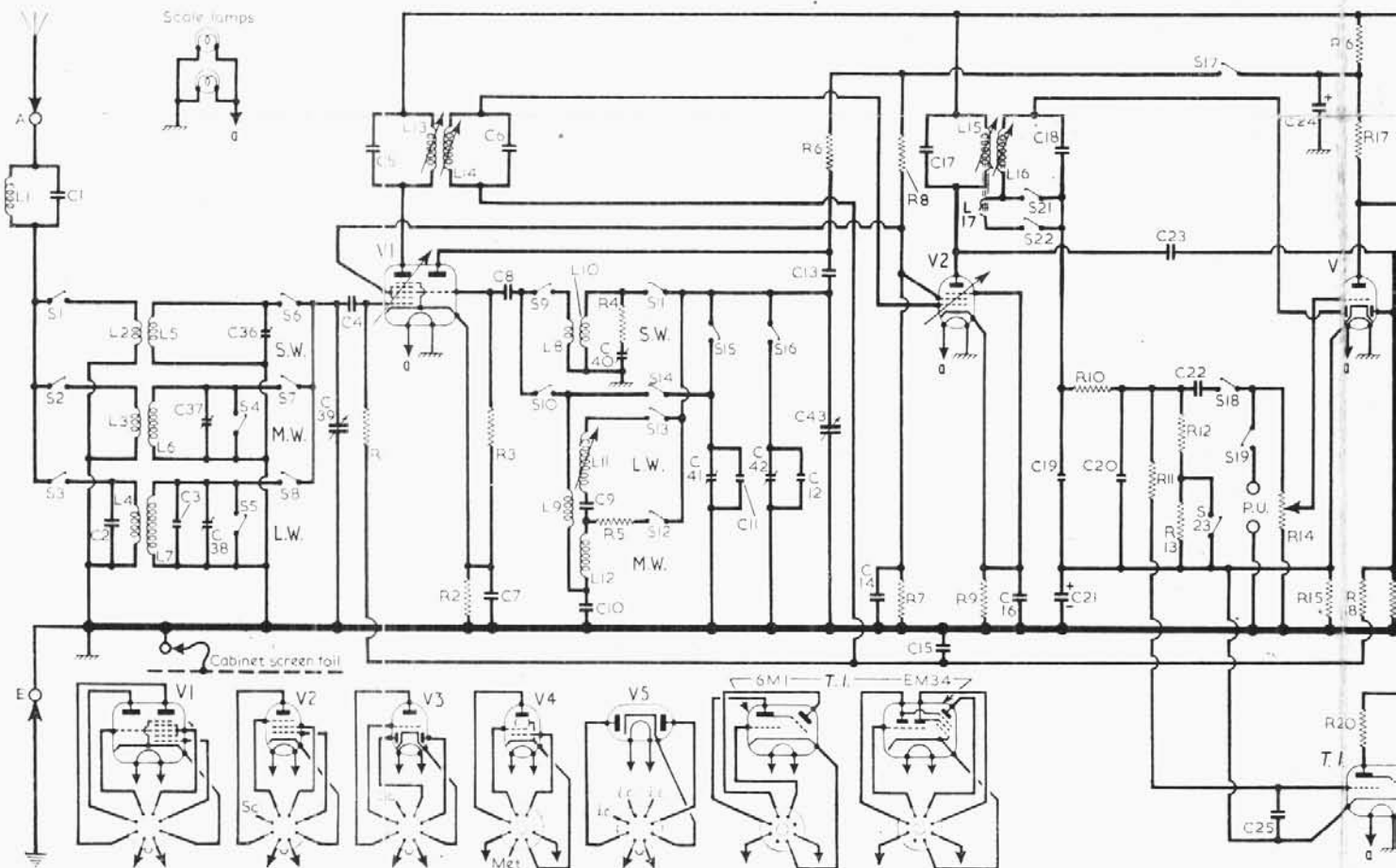
Circuit diagram of the Murphy A170 receiver, as produced at Welwyn. Another version, produced at Dublin, contains two small differences which are explained overleaf under "Modifications". The temperature fuse in the mains transformer circuit melts if the transformer over
