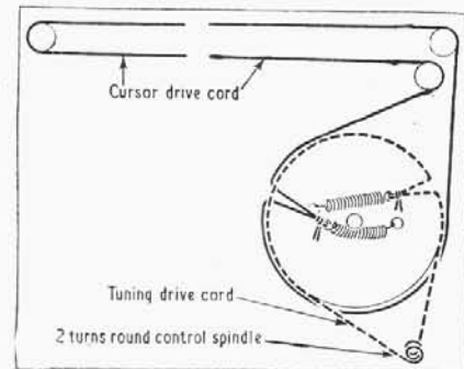
Sketch of the tuning drive system, as seen from the front, with gang at maximum.
